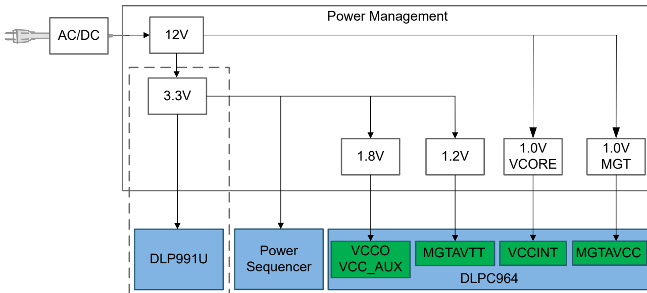
Figure 7-11. Power Distribution
