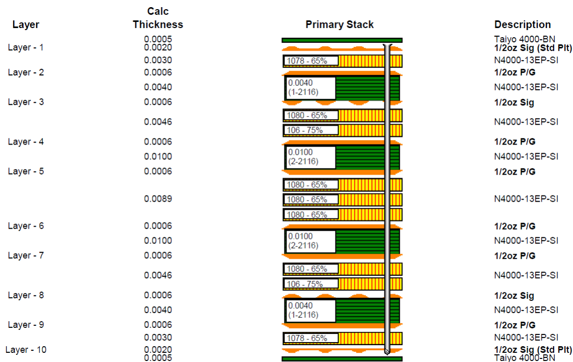
Figure 7-14. PCB Stack-Up
