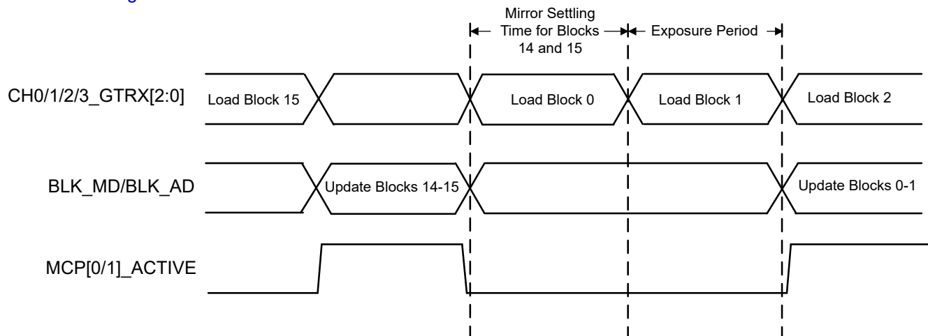
Figure 6-6. Dual Block Load Phased Sequence
