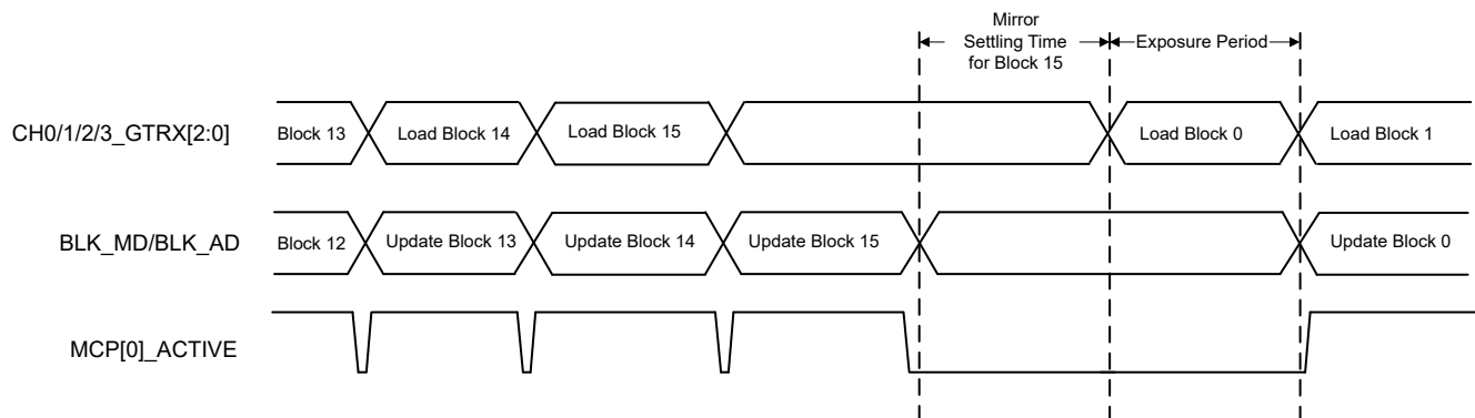
Figure 6-5. Single Block Load Phased Sequence
