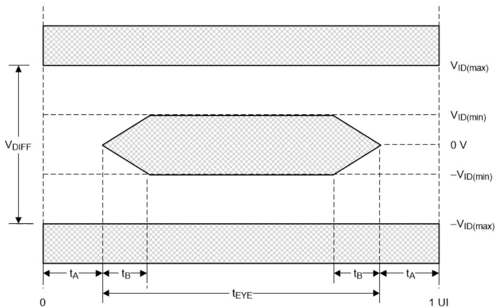
Figure 6-8. V-by-One Timing
