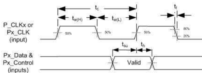
Figure 6-6. Port1, Port2, and Port3 Input Interface
