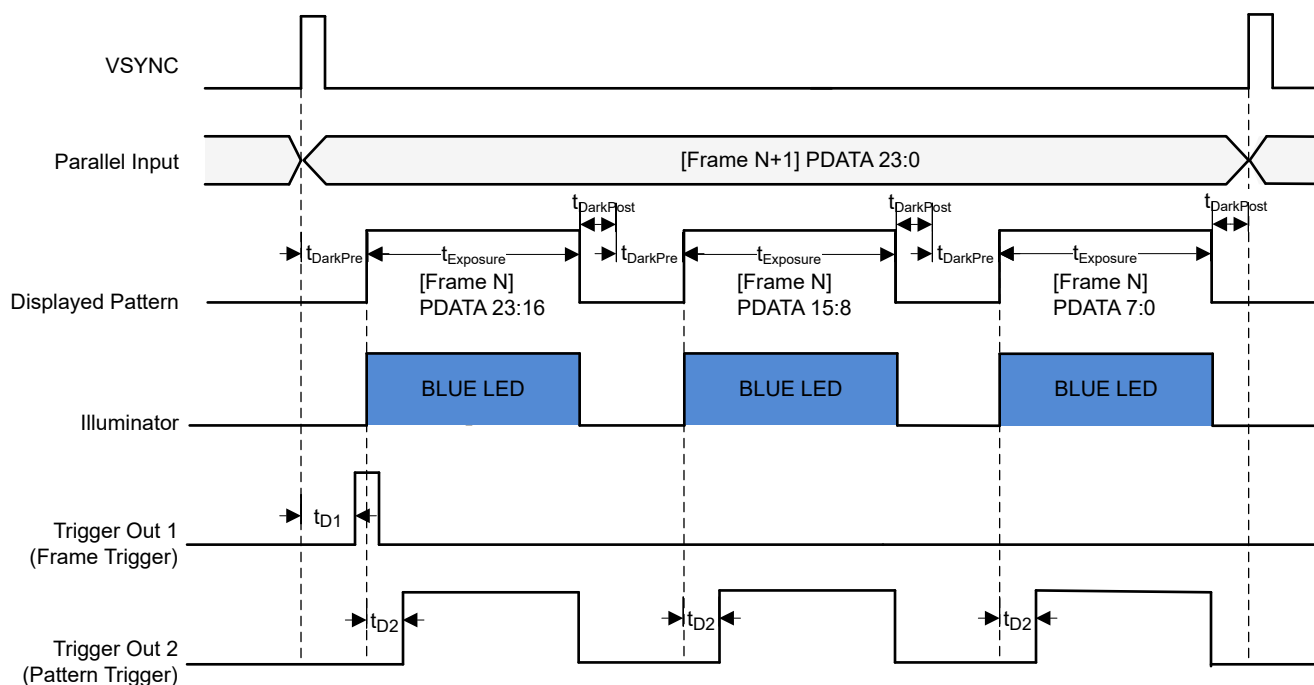
Figure 7-8. 3 × 8-bit (Blue) Pattern Configurations
