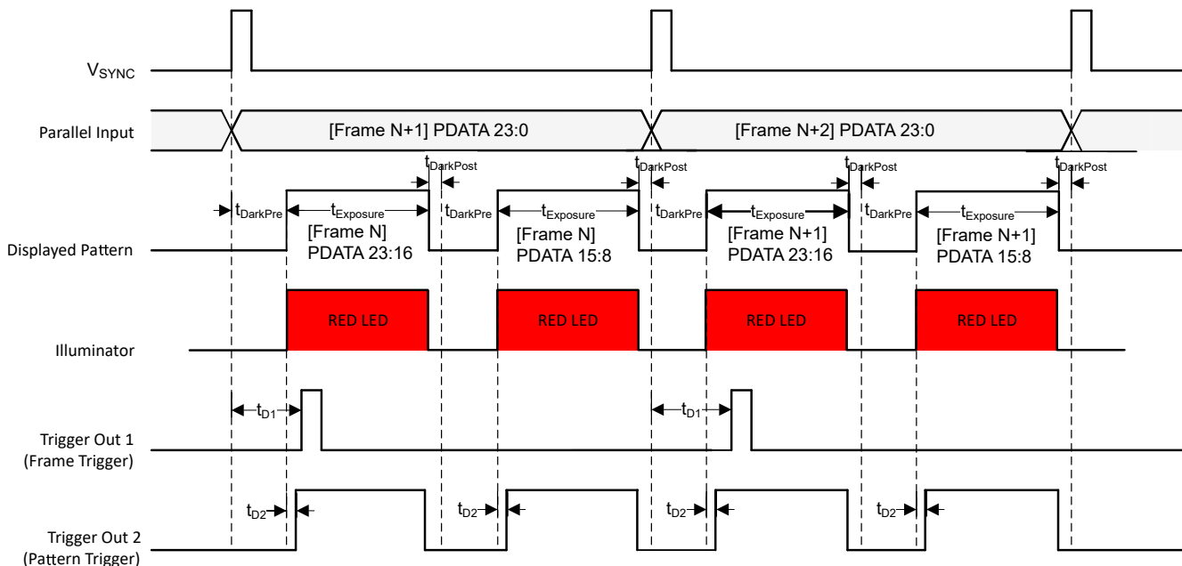
Figure 7-9. 2 \times 8 -bit (Red) Pattern Configurations
