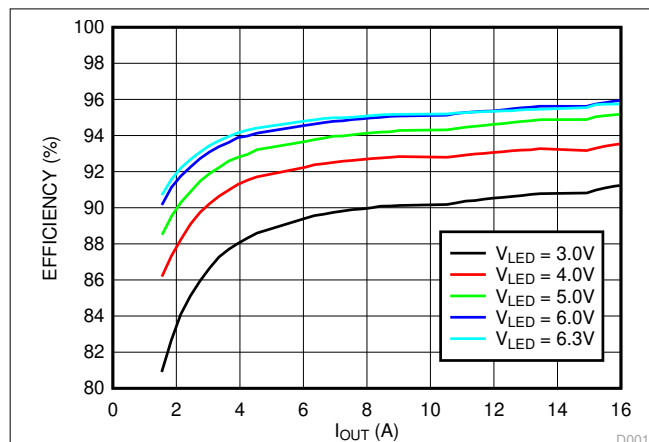
Figure 7-10. Illumination Driver Plus Power FETs Efficiency ( V_{ILLUM\_A\_IN} = 12 V )
