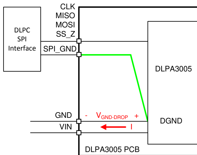
Figure 10-2. SPI Connections
