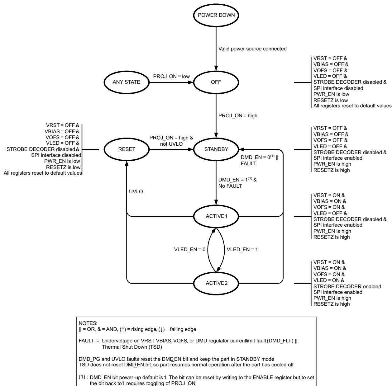
Figure 11. State Diagram
