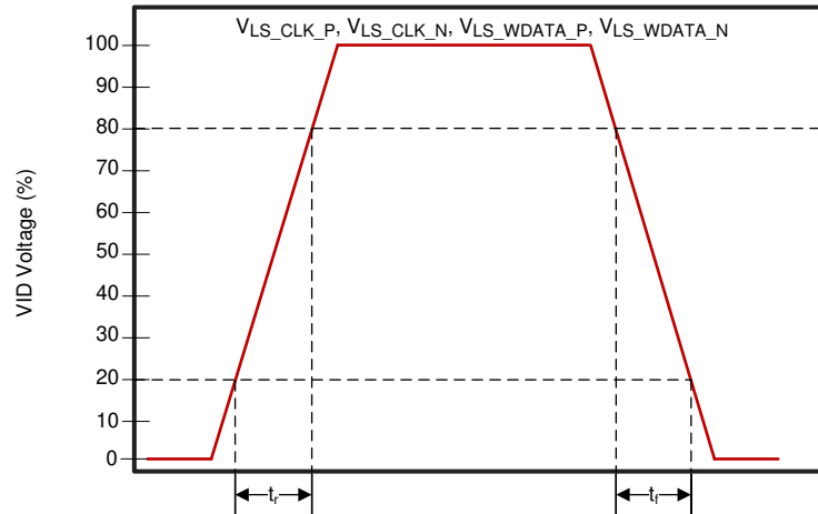
Figure 5-5. LSIF Rise, Fall Time Slew
