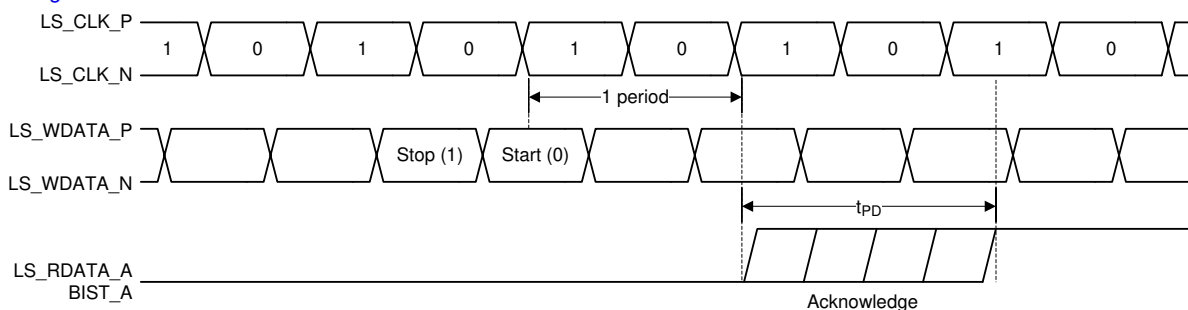
Figure 5-2. Switching Characteristics
