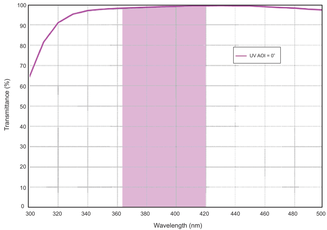
Figure 9-3. Corning 7056 Nominal UV Window Transmittance (Maximum Transmission Region)
