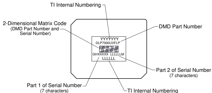
Figure 12-2. Device Marking
