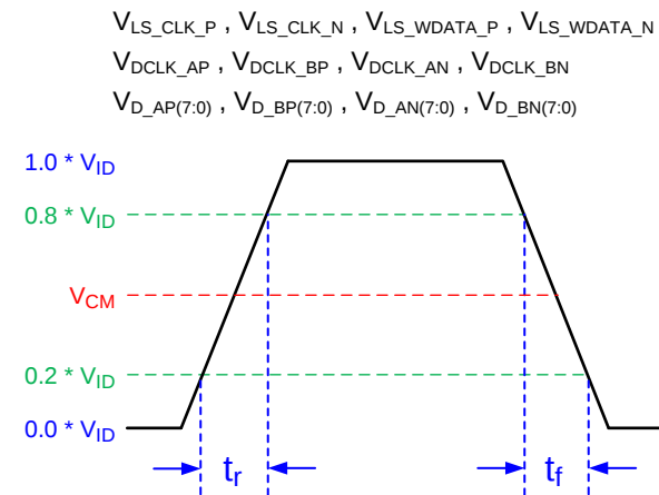
Figure 3. SubLVDS Input Rise and Fall Slew Rate
