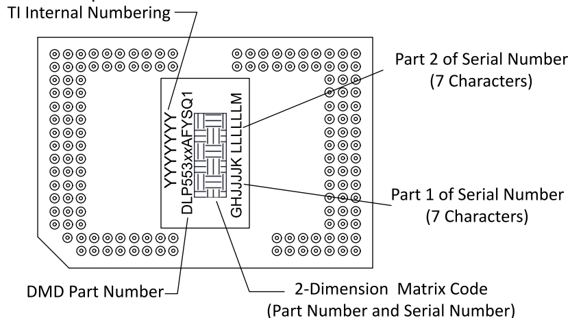
Figure 11-2. DMD Marking
