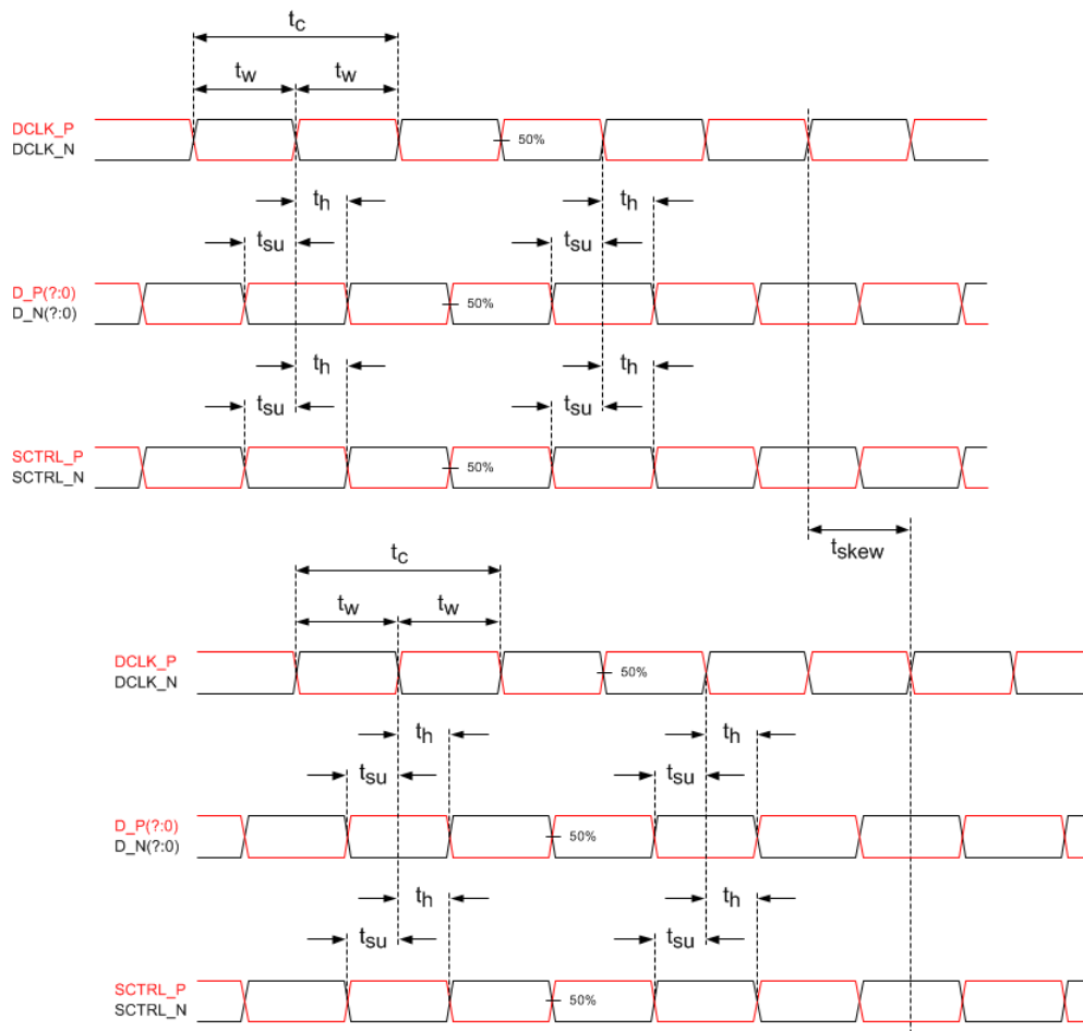
Figure 5-5. Timing Requirements
