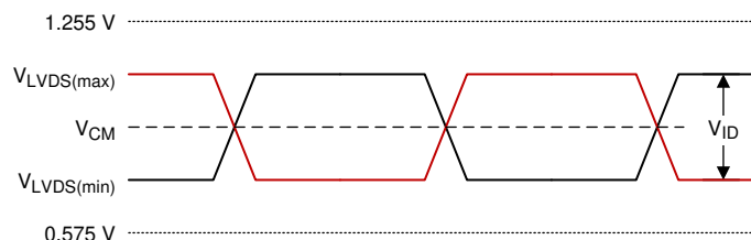
Figure 5-3. LSIF Waveform Requirements
