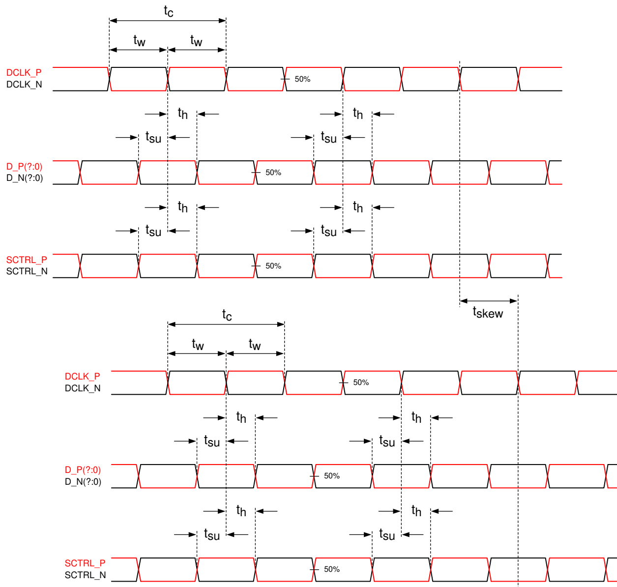
Figure 5-6. Timing Requirements
