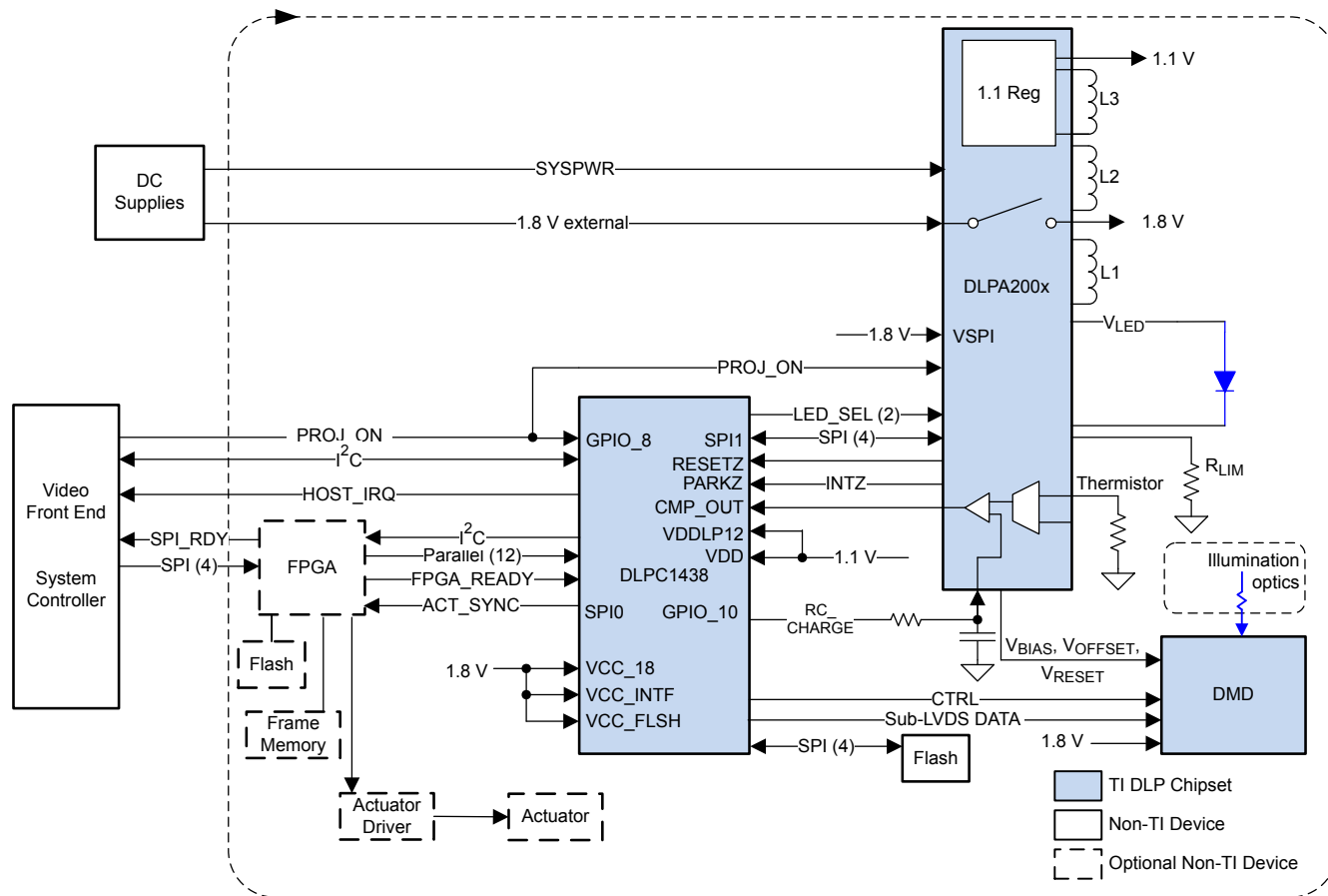
Figure 8-1. With FPGA
