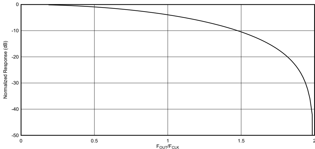
Figure 7-10. DES Output Frequency Response
