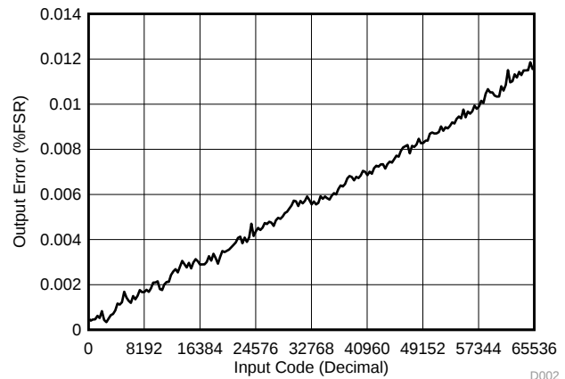
Figure 37. Input Code vs Output Error
