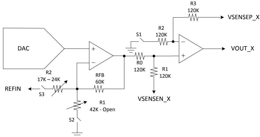
Figure 102. Voltage Output
