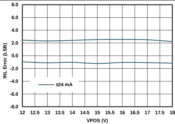
Figure 17. IOU T Linearity Error vs Power Supplies
