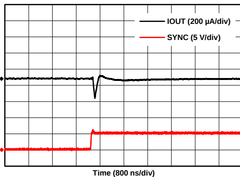
Figure 26. IOUT Full-Scale Settling Time, Falling Edge
