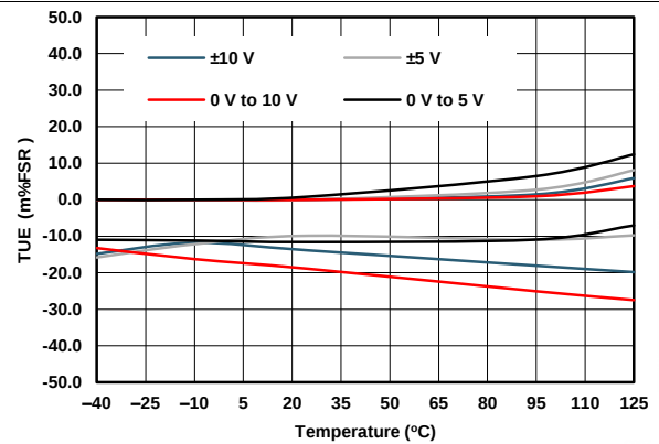
Figure 49. VOUT Total Unadjusted Error vs Temperature
