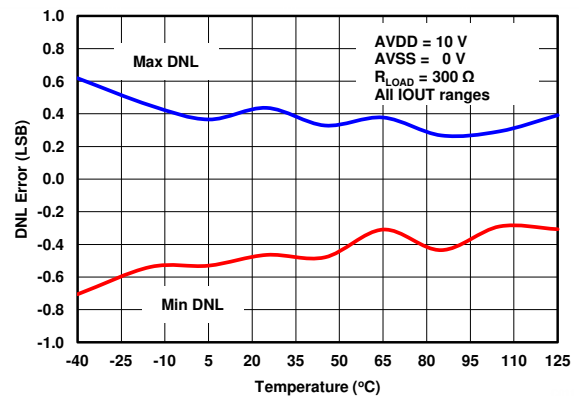
Figure 7-64. IOU DNL vs Temperature (External R_{SET} )
