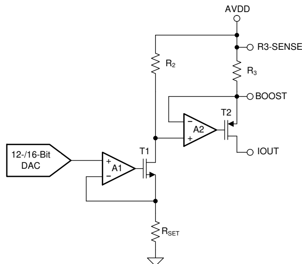
Figure 8-2. Current Output
