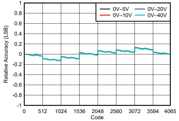
Figure 5-11. DAC61401 Relative Accuracy vs Digital Input Code (Unipolar Outputs)
