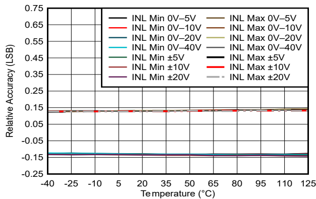
Figure 5-16. DAC81401 Relative Accuracy vs Temperature
