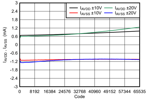
Figure 5-28. Supply Current ( I_{AVDD} , I_{AVSS} ) vs Digital Input Code
