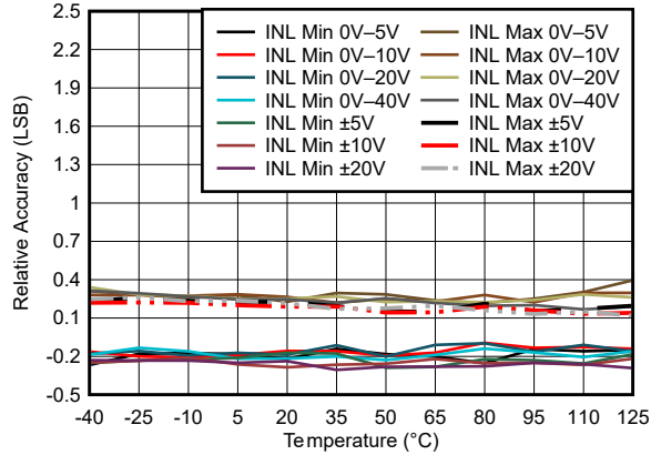
Figure 5-16. DAC81401 Relative Accuracy vs Temperature
