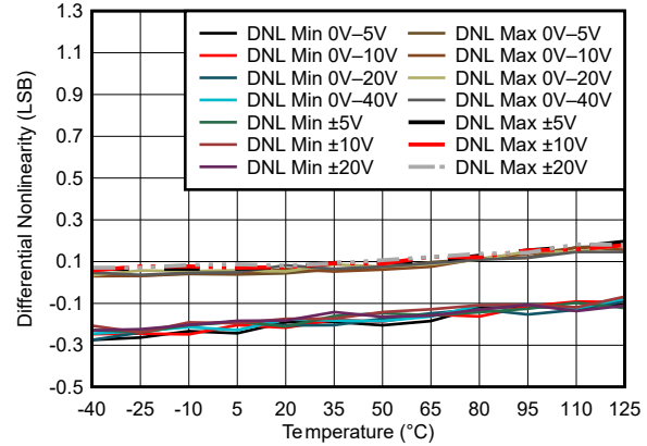
Figure 5-17. DAC81401 DNL vs Temperature
