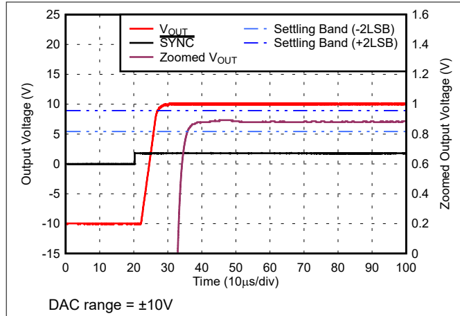
Figure 5-34. Full-Scale Settling Time, Rising Edge
