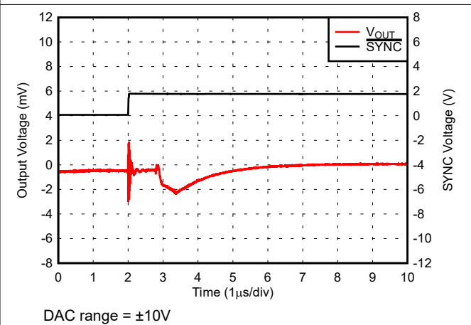
Figure 5-37. Glitch Impulse, 1LSB Step, Rising Edge
