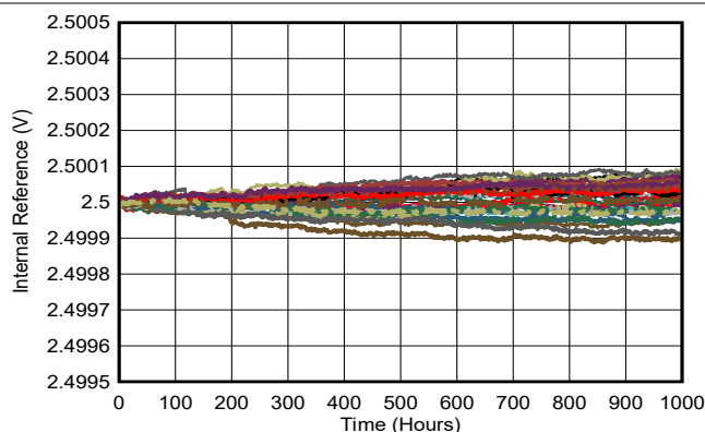
Figure 5-47. Internal Reference Voltage vs Time (WQFN)
