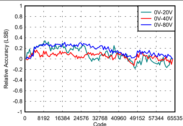
Figure 8-4. Relative Accuracy vs Digital Input Code (Unipolar Mode)
