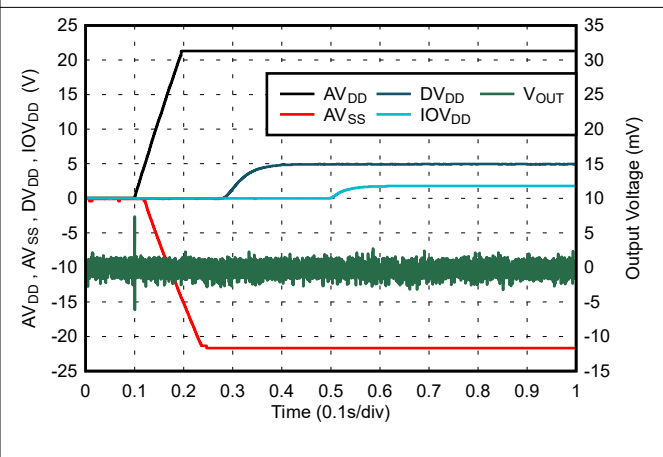
Figure 5-39. Power-Up Response
