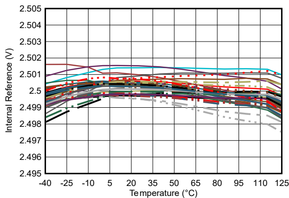
Figure 5-44. Internal Reference Voltage vs Temperature (TSSOP)
