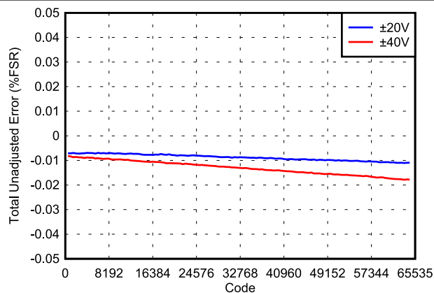
Figure 8-7. TUE vs Digital Input Code (Bipolar Mode)
