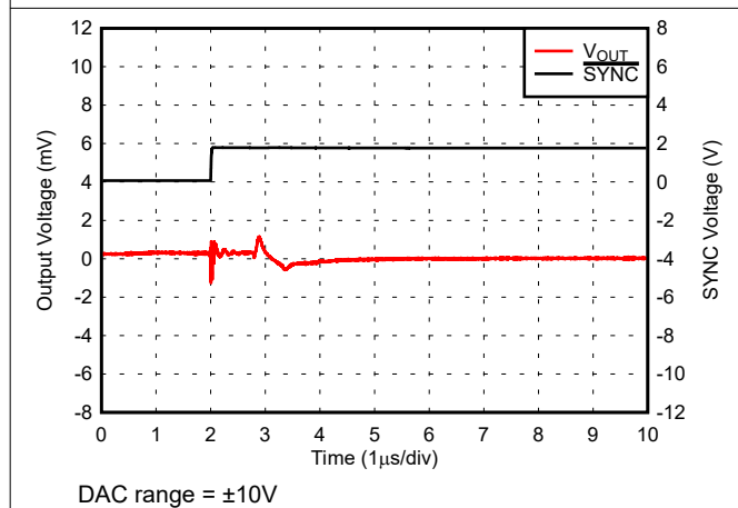
Figure 5-38. Glitch Impulse, 1LSB Step, Falling Edge
