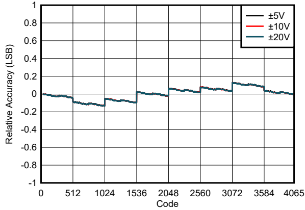
Figure 5-10. DAC61401 Relative Accuracy vs Digital Input Code (Bipolar Outputs)
