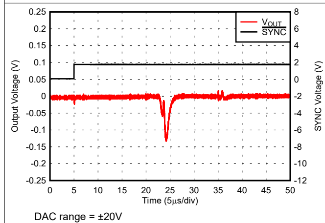
Figure 5-36. DAC Output Enable Glitch
