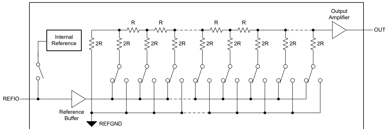
Figure 6-1. DACx1401 R-2R Ladder DAC
