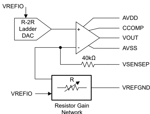
Figure 6-2. DACx1401 Voltage Output
