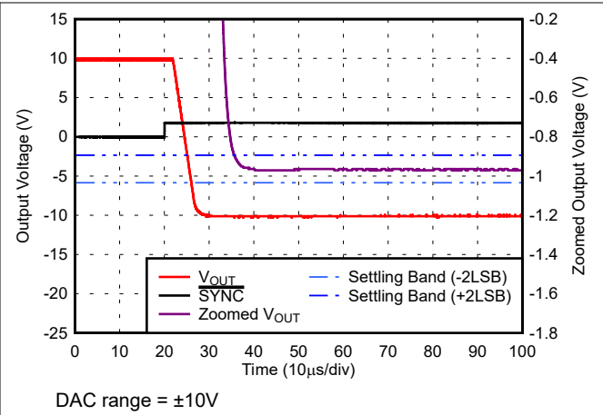
Figure 5-35. Full-Scale Settling Time, Falling Edge
