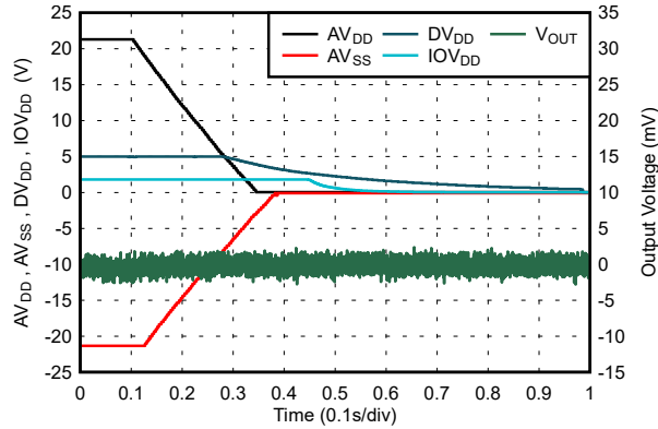
Figure 5-40. Power-Down Response
