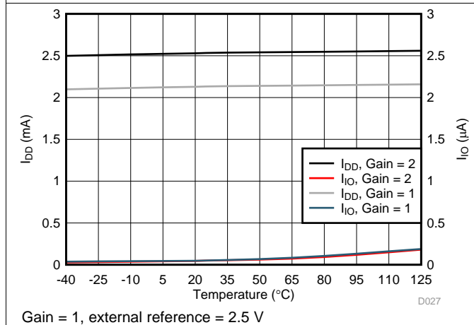
Figure 27. Supply Current With External Reference vs Temperature
