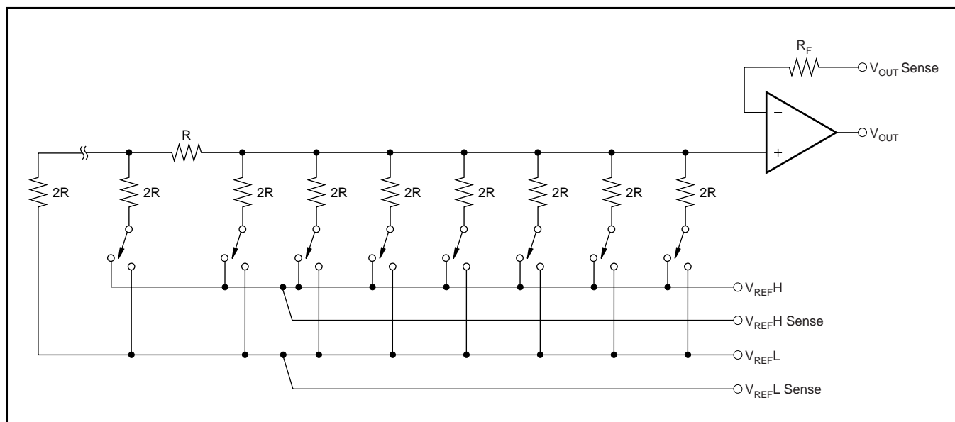
FIGURE 1. DAC7632 Architecture.
