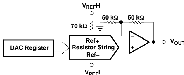
Figure 29. R-String DAC Architecture
