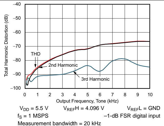
Figure 25. Total Harmonic Distortion vs Output Frequency
