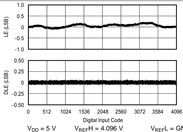
Figure 2. Linearity Error and Differential Linearity Error vs Digital Input Code
