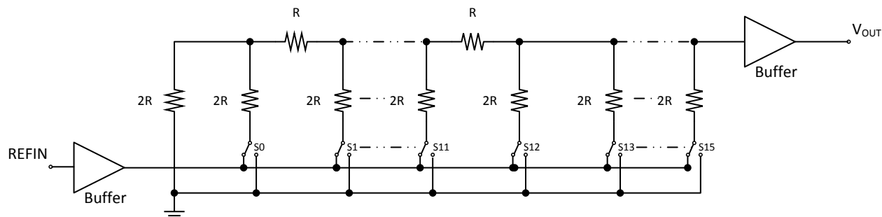
Figure 51. DACx0004 Architecture
