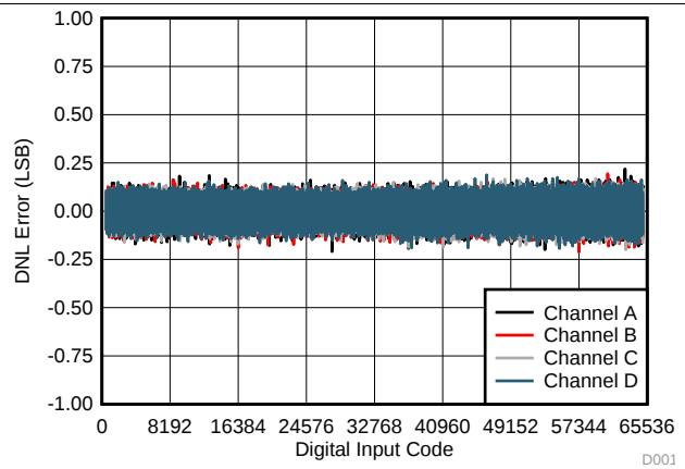
Figure 16. Differential Linearity Error vs Digital Input Code
