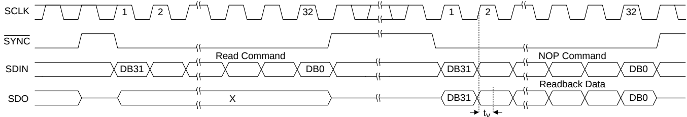
Figure 54. Read-Back Operation
