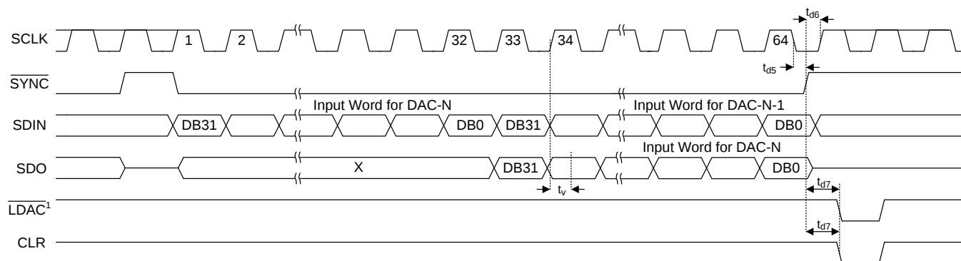
Figure 2. Daisy-Chain Timing
