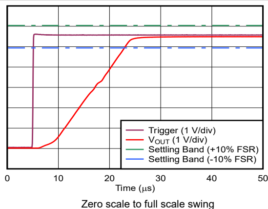
Figure 5-21. Voltage Output Setting Time: Rising Edge
