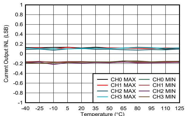
Figure 6-32. Current Output INL vs Temperature
