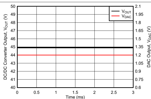
Figure 8-3. Nominal Voltage Output
