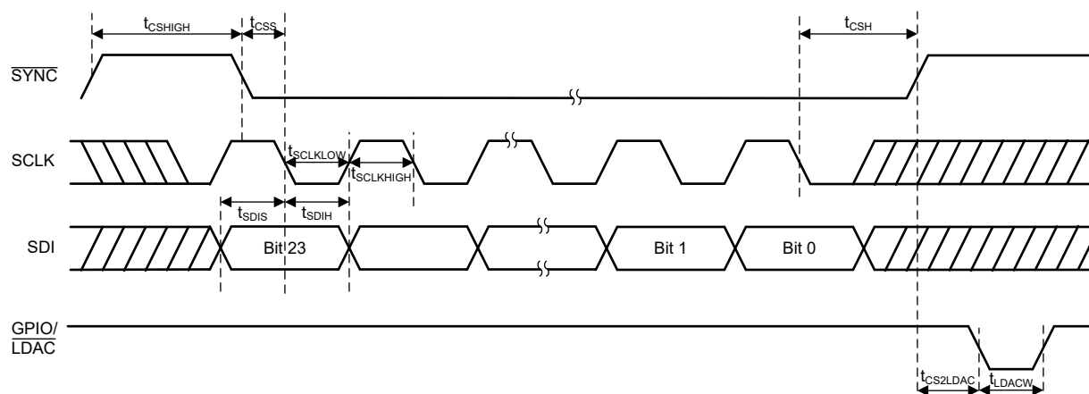
Figure 5-2. SPI Write Timing Diagram
