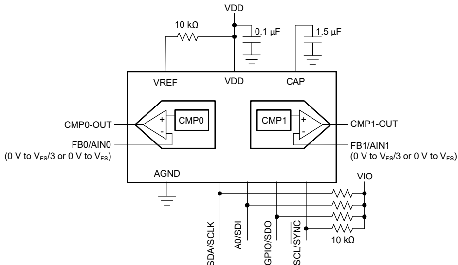
Figure 6-3. Comparator Interface
