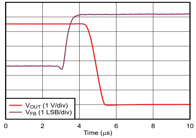
Figure 5-50. Comparator Response Time: High-to-Low Transition
