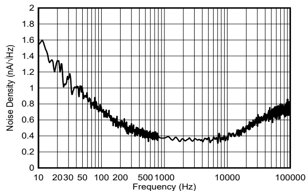
Figure 6-56. Current Output Noise Density
