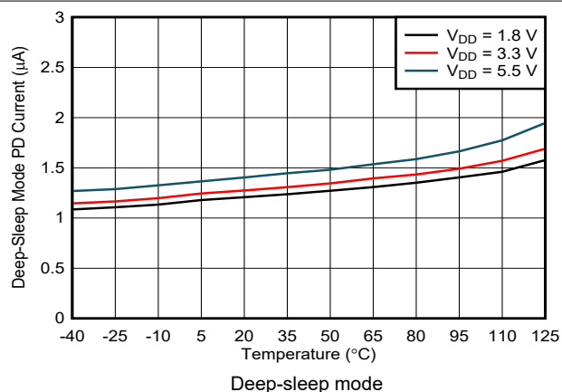
Figure 6-65. Power-Down Current vs Temperature
