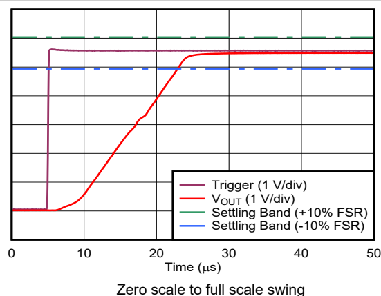
Figure 6-21. Voltage Output Setting Time: Rising Edge
