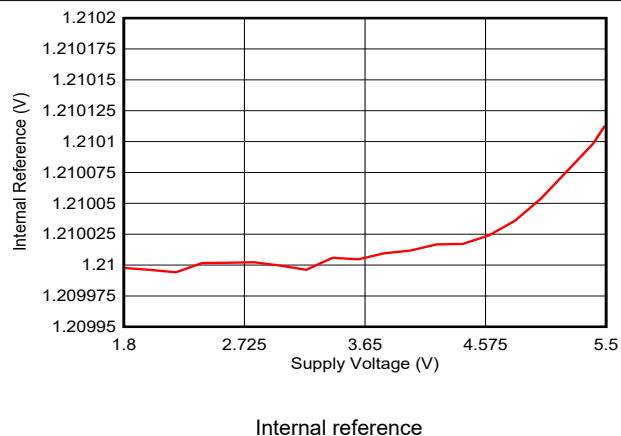
Figure 6-63. Internal Reference vs Supply Voltage
