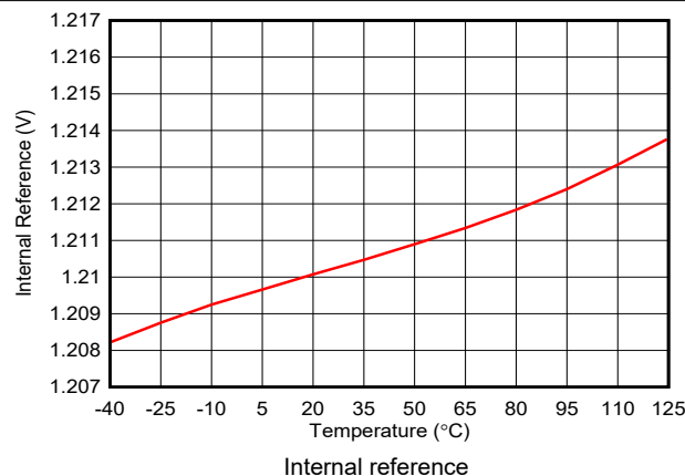
Figure 6-62. Internal Reference vs Temperature
