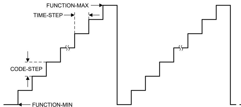
Figure 7-13. Sawtooth Waveform
