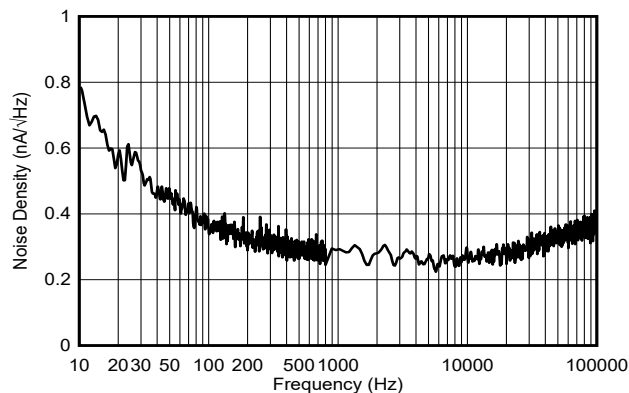
Figure 6-55. Current Output Noise Density
