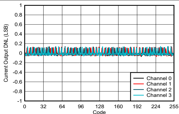
Figure 6-38. Current Output DNL vs Digital Input Code
