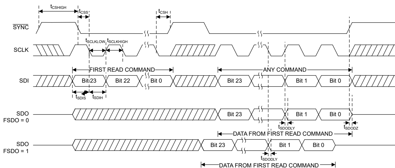
Figure 6-3. SPI Read Timing Diagram
