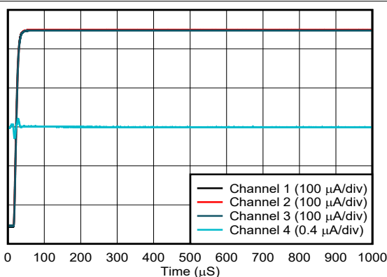
Figure 6-51. Current Output Power-On Glitch
