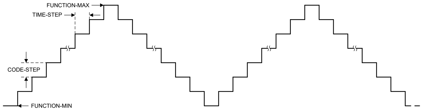
Figure 7-12. Triangle Waveform
