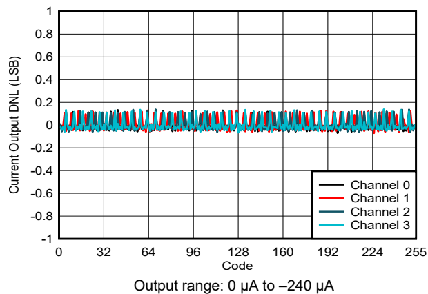
Figure 6-38. Current Output DNL vs Digital Input Code
