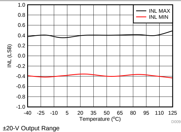
Figure 9. Integral Linearity Error vs Temperature
