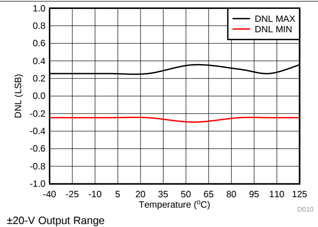
Figure 10. Differential Linearity Error vs Temperature
