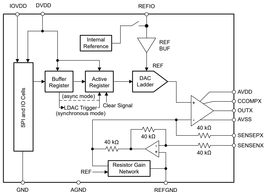
Figure 8-1. Device Architecture
