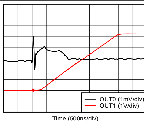
Figure 5-36. AV_{DD} Power Down Response
