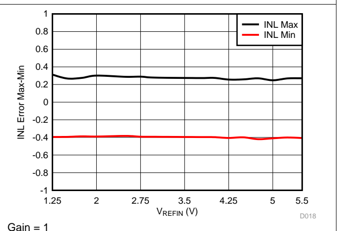
Figure 18. Integral Linearity Error vs Reference Voltage
