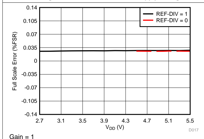
Figure 17. Full Scale Error vs Supply Voltage
