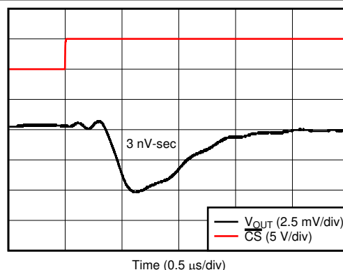
DAC code transition from midscale – 1 to midscale LSB, REF-DIV = 0 and BUFF-GAIN = 0 Figure 7-36. Glitch Impulse, Rising Edge, 1-LSB Step
