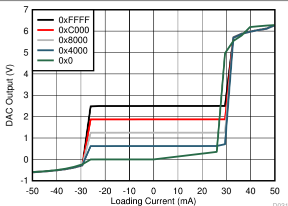
REF-DIV = 0 and BUFF-GAIN = 0 Figure 7-33. Source and Sink Capability
