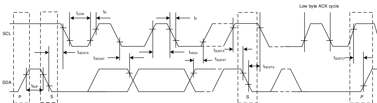
Figure 7-2. I 2 C Mode Timing
