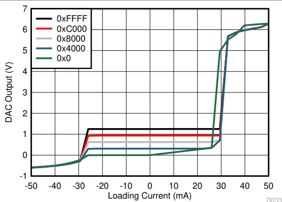
REF-DIV = 1 and BUFF-GAIN = 0 Figure 7-35. Source and Sink Capability
