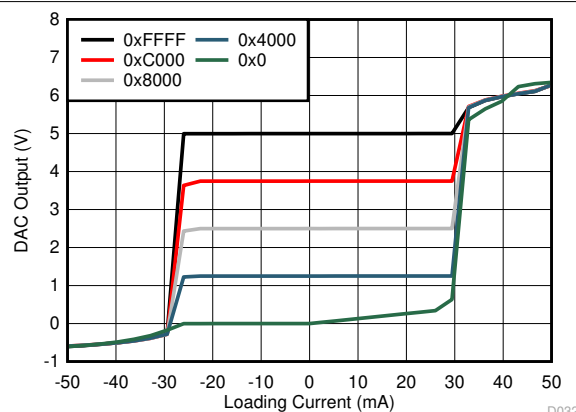
REF-DIV = 0 and BUFF-GAIN = 1 Figure 7-34. Source and Sink Capability
