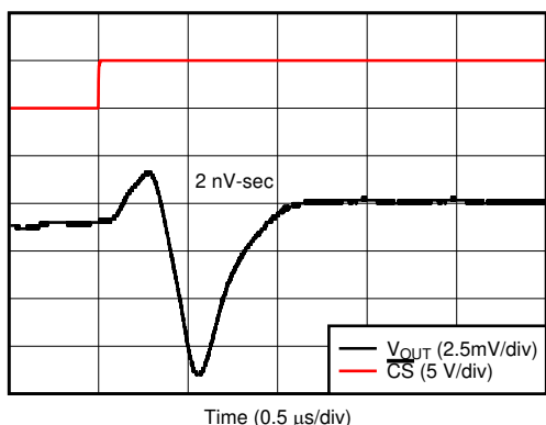
DAC code transition from midscale to midscale – 1 LSB, REF-DIV = 0 and BUFF-GAIN = 0 Figure 7-37. Glitch Impulse, Falling Edge, 1-LSB Step
