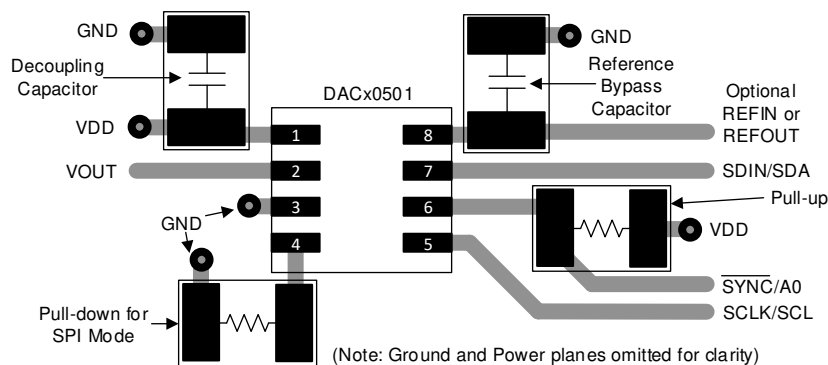
Figure 9-3. Layout Example
