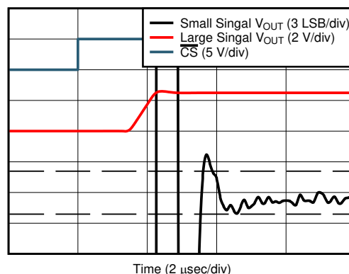
REF-DIV = 0 and BUFF-GAIN = 0 Figure 7-38. Full-Scale Settling Time, Rising Edge
