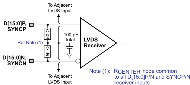
Figure 30. D[15:0]P/N and SYNC/N LVDS Input Configuration
