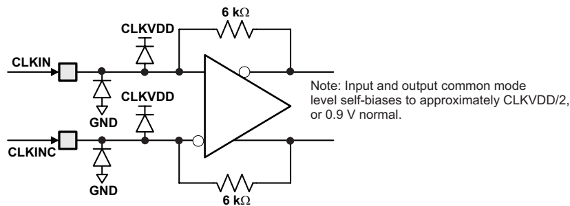
Figure 45. CLKIN/C Equivalent Input Circuit
