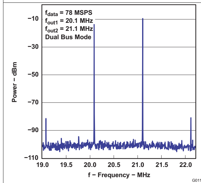
Figure 11. Two-Tone Spectrum
