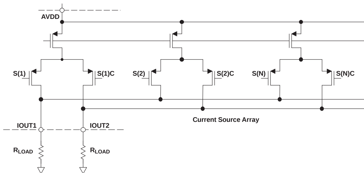
Figure 19. Analog Outputs
