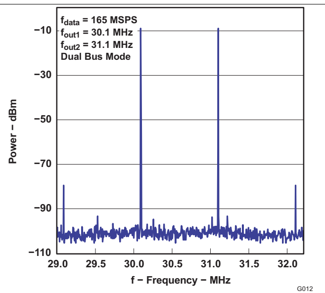
Figure 12. Two-Tone Spectrum
