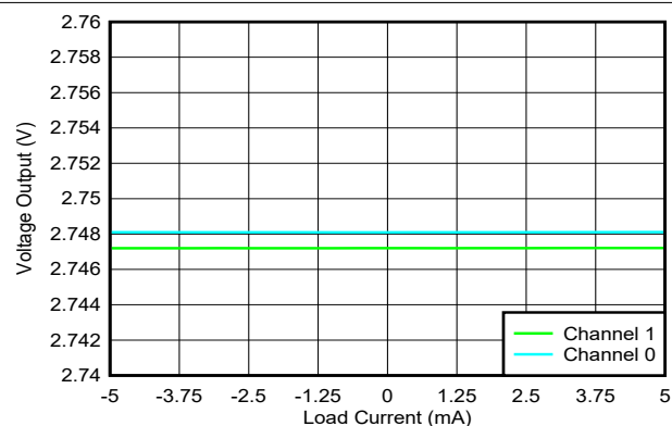
Figure 6-18. Voltage Output vs Load Current DAC channels at midscale
