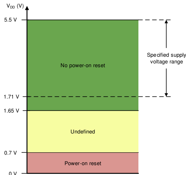
Figure 7-6. Threshold Levels for V_{DD} POR Circuit
