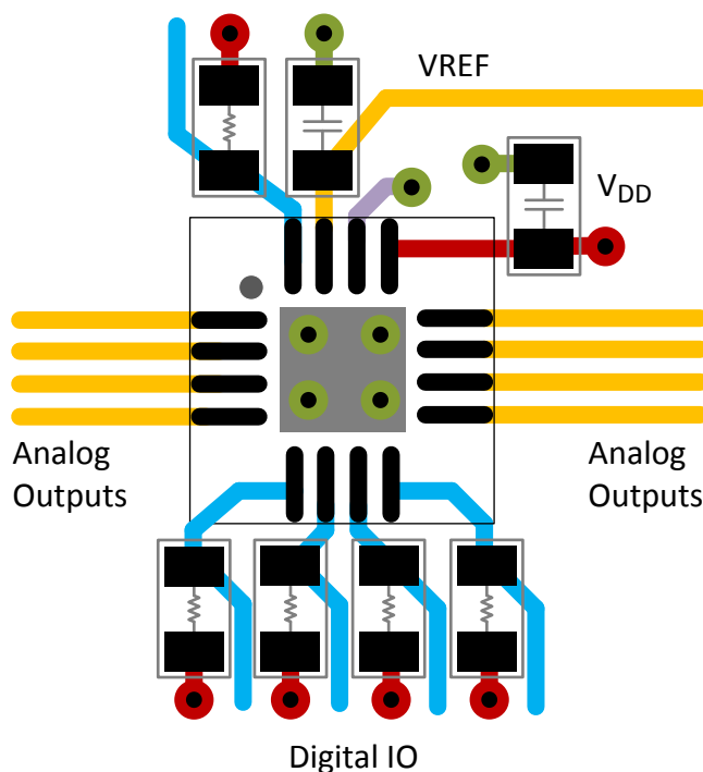
Figure 68. Layout Example
