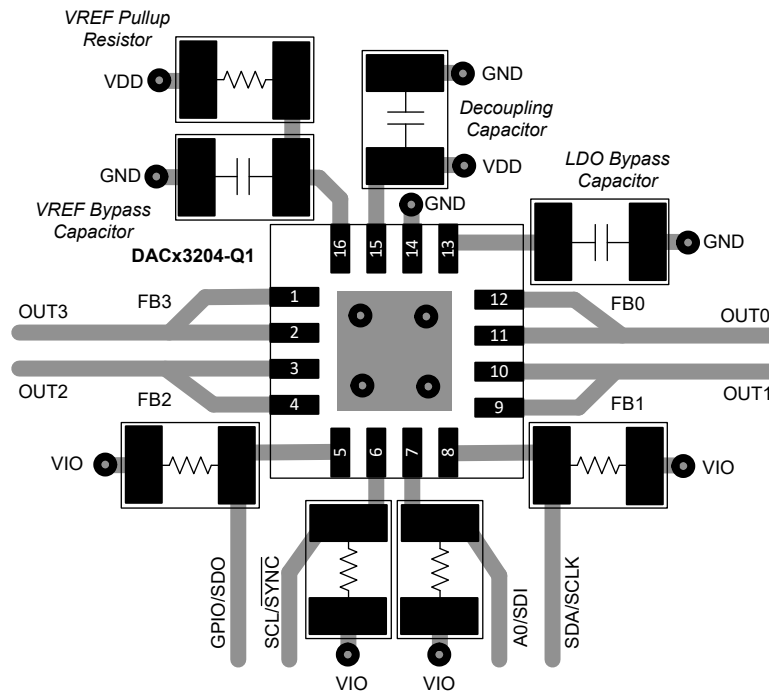
Figure 8-4. Layout Example
