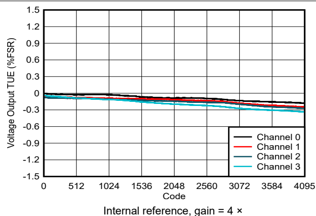
Figure 6-12. Voltage Output TUE vs Digital Input Code
