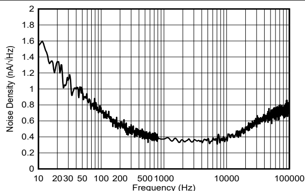
Figure 6-49. Current Output Noise Density
