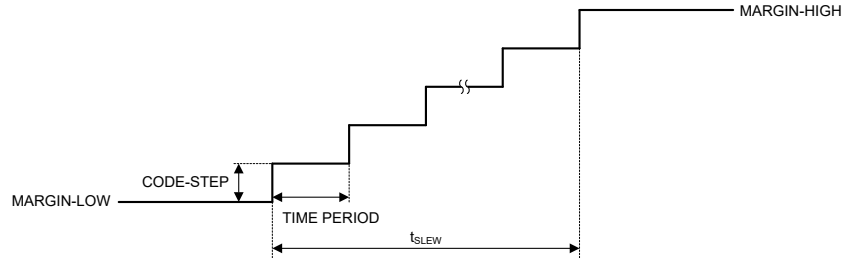
Figure 7-10. Programmable Slew-Rate Control
