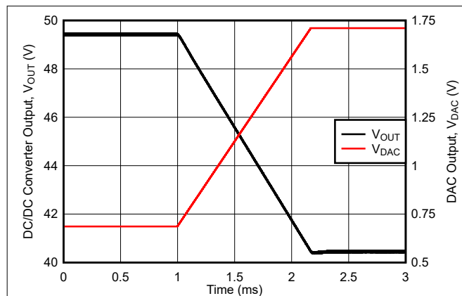
Figure 8-2. Margin-High to Margin-Low Transition
