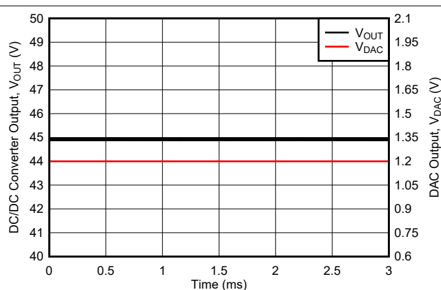
Figure 8-3. Nominal Voltage Output
