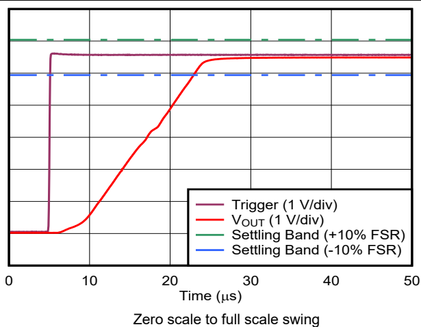
Figure 6-21. Voltage Output Settling Time - Rising Edge
