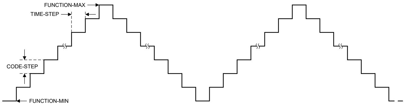
Figure 7-12. Triangle Waveform
