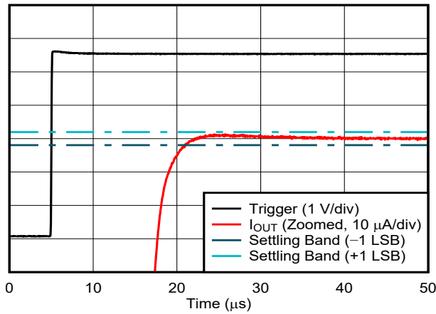
Figure 6-43. Current Output Setting Time, Rising Edge
