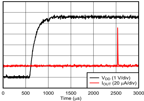
DAC at mid scale ( 0\text{ }\mu\text{A} ) stored in EEPROM Figure 6-45. Current Output Power-On Glitch
