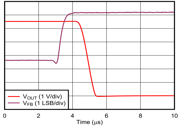
Figure 6-52. Comparator Response Time: High-to-Low Transition
