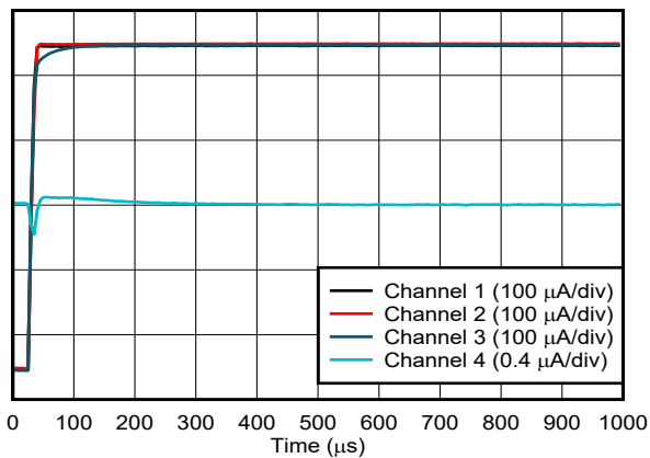
Channel 4 is victim, all other channels are aggressors Figure 6-47. Current Output Channel-to-Channel Crosstalk
