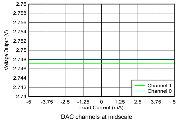
Figure 6-18. Voltage Output vs Load Current
