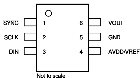
Figure 6-1. DCK Package, 6-Pin SC70 (Top View)
