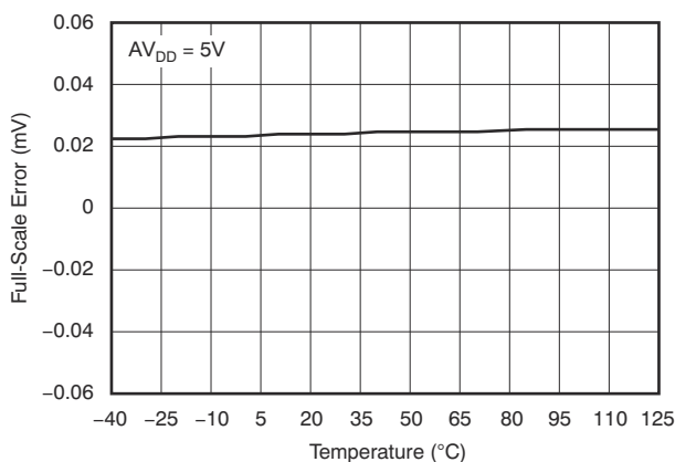
Figure 7-13. Full-Scale Error vs Temperature
