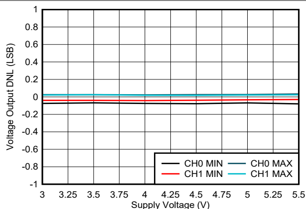
Figure 5-11. Voltage Output DNL vs Supply Voltage
