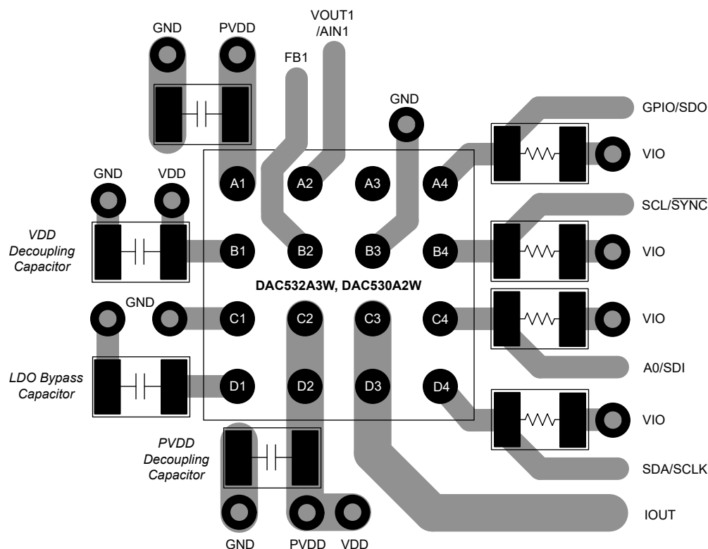
Figure 8-4. Layout Example
