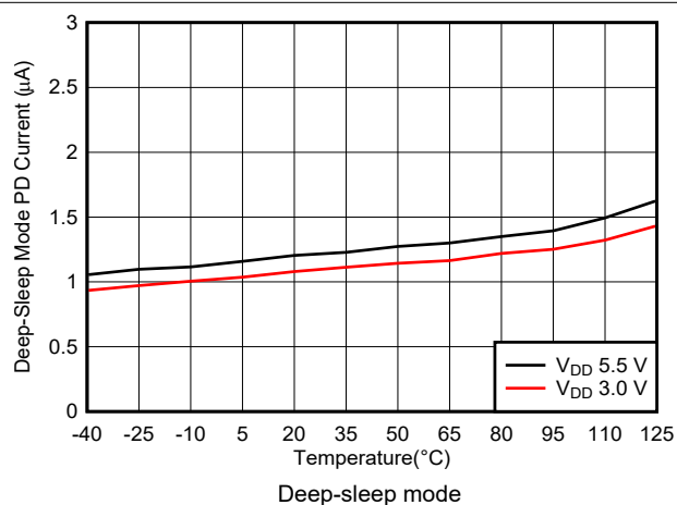
Figure 5-56. Power-Down Current vs Temperature
