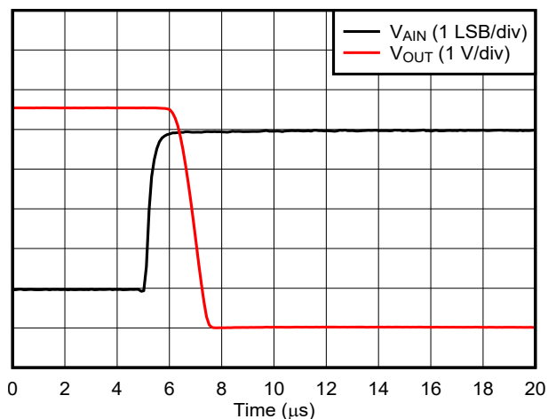
Comparator output in push-pull mode Figure 5-51. Comparator Response Time: High-to-Low Transition
