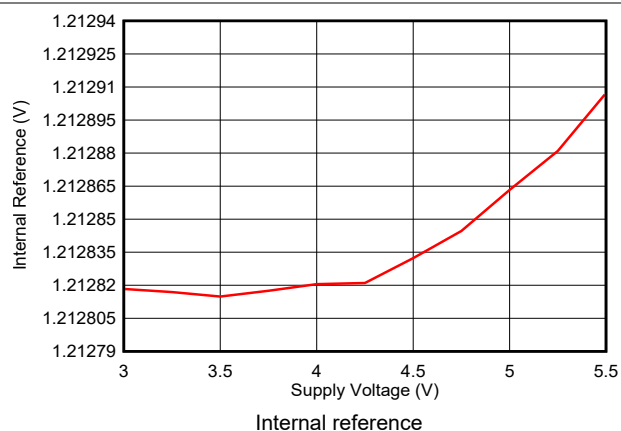
Figure 5-54. Internal Reference vs Supply Voltage
