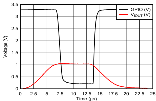
Figure 8-3. Comparator Toggle
