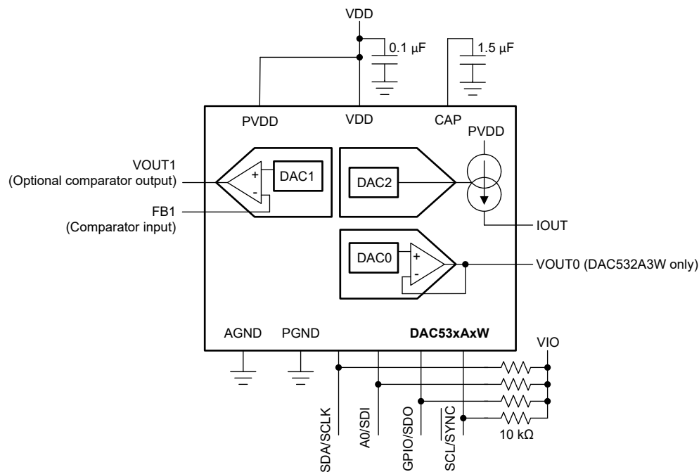
Figure 6-2. Comparator Interface
