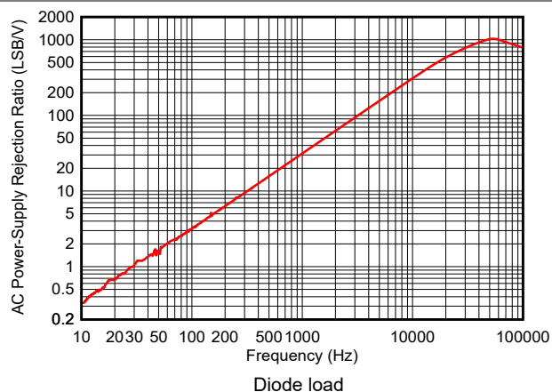
Figure 5-48. Current Output AC PSRR vs Frequency
