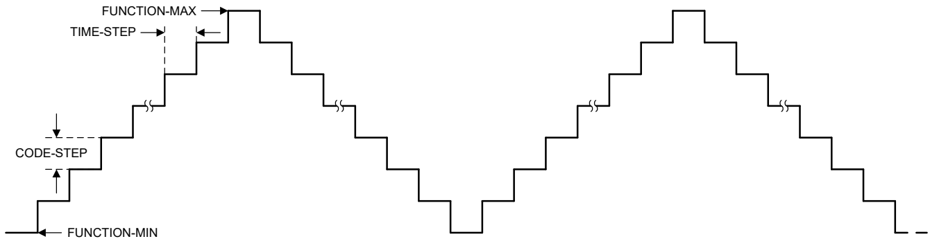
Figure 6-10. Triangle Waveform
