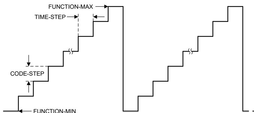
Figure 6-11. Sawtooth Waveform
