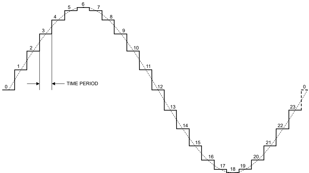
Figure 6-12. Sine Wave Generation
