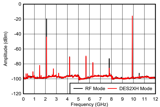
includes PCB, cable and balun loss Figure 6-34. f_{\text{OUT}} = 9897\text{ MHz} , 0 dBFS
