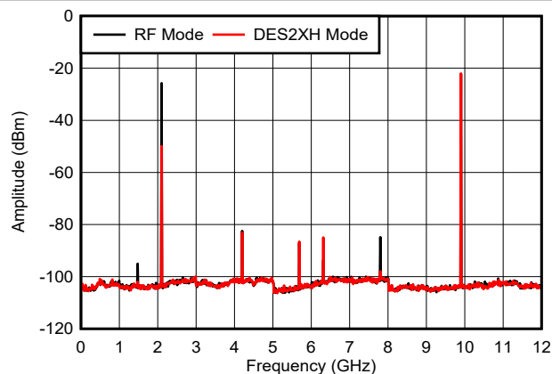
includes PCB, cable and balun loss Figure 6-35. f_{\text{OUT}} = 9897\text{ MHz} , -6 dBFS
