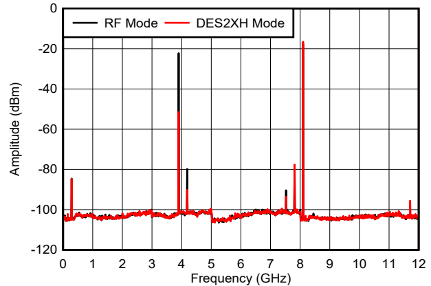
includes PCB, cable and balun loss Figure 6-32. f_{\text{OUT}} = 8097\text{ MHz} , -6 dBFS
