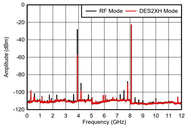
includes PCB, cable and balun loss Figure 6-33. f_{\text{OUT}} = 8097\text{ MHz} , -12 dBFS
