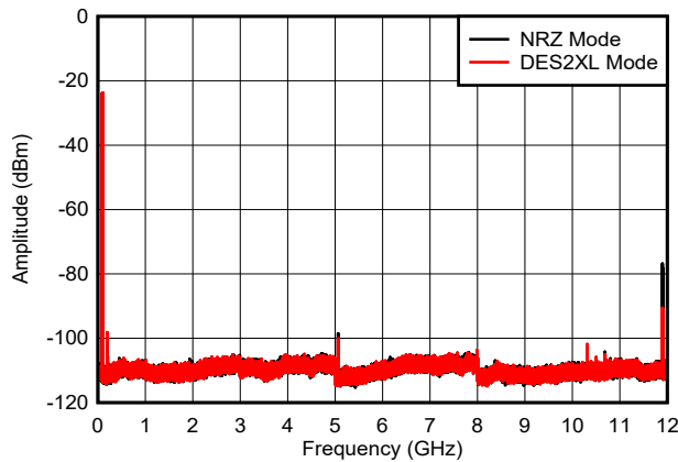
Figure 6-41. Dual Tone, f_{\text{OUT}} = 97\text{ MHz} , -12 dBFS (0 - f_{\text{CLK}} )
