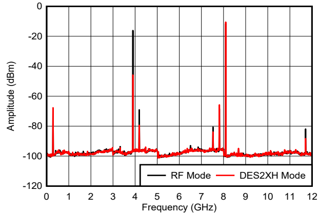
includes PCB, cable and balun loss Figure 6-31. f_{\text{OUT}} = 8097\text{ MHz} , 0 dBFS
