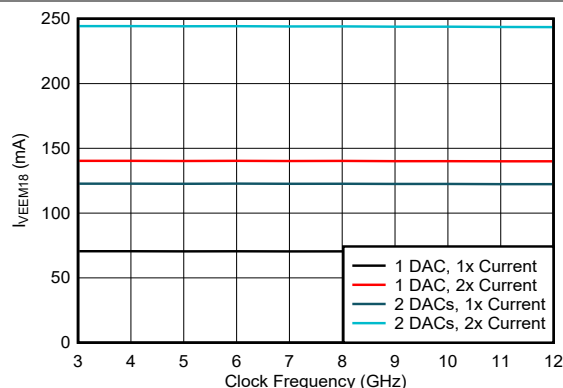
Figure 6-210. VEEM18 Current vs Clock Frequency and DAC Mode
