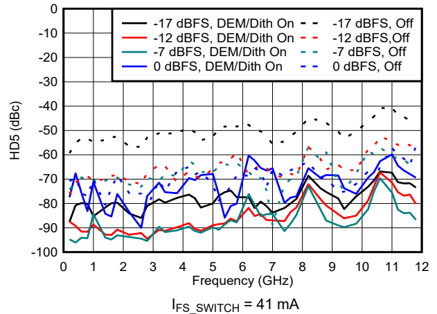
Figure 6-179. HD5 vs Frequency and Digital Amplitude in NRZ/RF Modes
