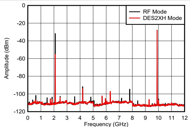
includes PCB, cable and balun loss Figure 6-36. f_{\text{OUT}} = 9897\text{ MHz} , -12 dBFS
