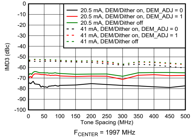
Figure 6-119. IMD3 vs Tone Spacing in DES2XL Mode
