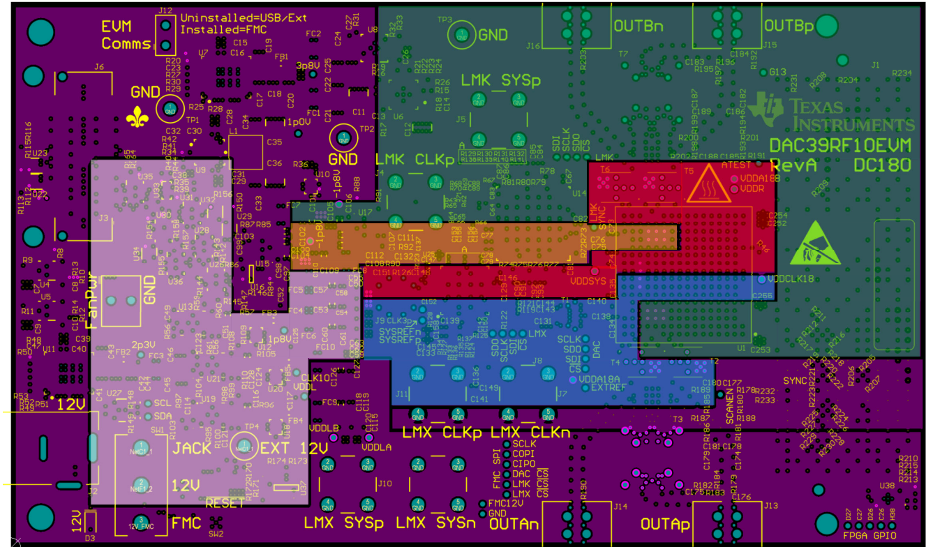
Layer12 / PWR3 DAC VDDA18A = RED DAC VDDA18B = ORANGE DAC VDDB = YELLOW DAC VEExA = GREEN DAC VEExB = BLUE VDDIO = WHITE Figure 8-33. Power Plane Layout for Layer 12
