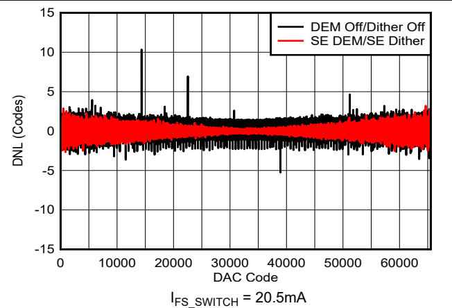
Figure 6-11. DNL vs DAC Code: 20.5mA
