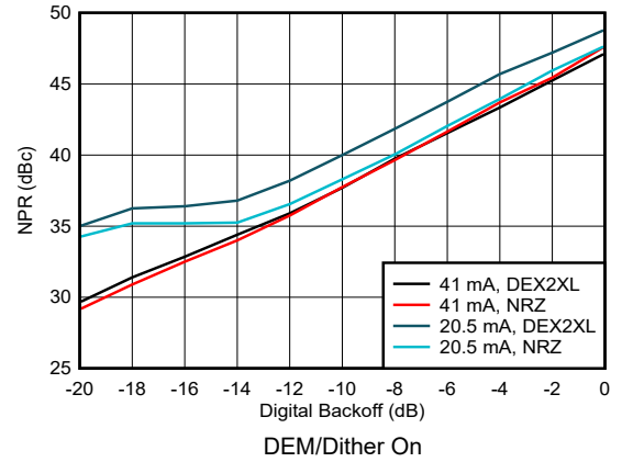
Figure 6-196. Noise Power Ratio vs Digital Backoff: 1 st Nyquist Zone
