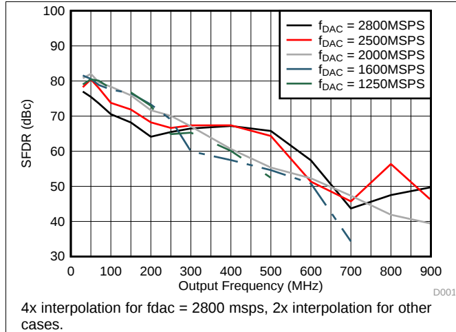
Figure 7. SFDR vs Output Frequency Over f_{DAC}
