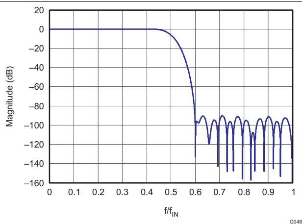
Figure 60. Magnitude Spectrum for FIR0
