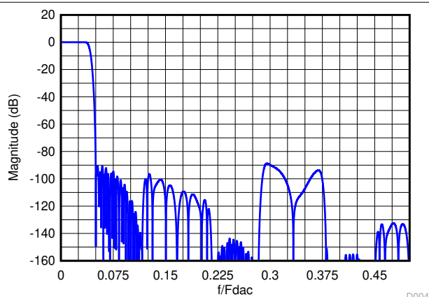
Figure 7-17. Composite Magnitude Response for 12x Interpolation
