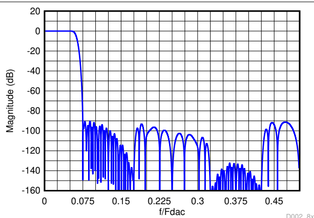
Figure 7-15. Composite Magnitude Response for 8x Interpolation
